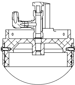
DETAIL E SCALE 1 : 3
